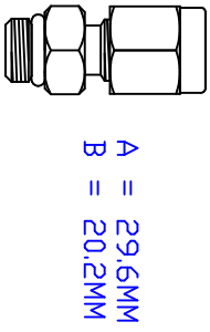
1/8" FITTING
